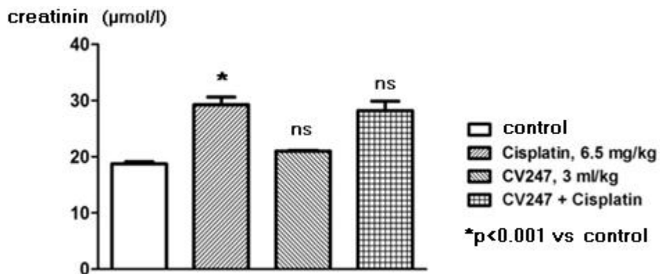
Figure 6. CV did not alter Cp caused azotaemia. (two-way ANOVA)
