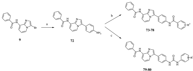
Figure 3. Synthesis of the para substituted imidazo[1,2- a ]pyridine derivatives. Reagents and conditions: (a) 4-(4,4,5,5-tetramethyl-1,3,2-dioxaborolan-2-yl)aniline, \text{Pd(PPh}_3)_4 , \text{Na}_2\text{CO}_3 , 1,4-dioxane, \text{H}_2\text{O} , microwave reactor, 140\text{ }^\circ\text{C} , 2 h, 36%; (b) benzoic acid derivative, EDCl, pyridine, 70\text{ }^\circ\text{C} , 2 h, 45-73%; (c) aryl isocyanate, anhydrous pyridine, 25\text{ }^\circ\text{C} , 2 h, 40-58%.
