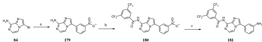
Figure 5. Synthesis of N -[3-(3-aminophenyl)imidazo[1,2- a ]pyrazine-8-yl]-3,5-bis(trifluoromethyl)benzamide ( 181 ). Reagents and conditions: (a) (3-nitrophenyl)boronic acid, Pd(PPh 3 ) 4 , Na 2 CO 3 , 1,4-dioxane, H 2 O, microwave reactor, 140 °C, 1.5 h, 57%; (b) 3,5-bis(trifluoromethyl)benzoic acid, EDCI, pyridine, 70 °C, 2 h, 36%; (c) H-Cube ® , column: 10% Pd/C, eluent: ethanol/ethyl acetate, 25 °C, 12%.
