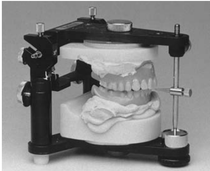
Fig. 14.9 (a) Acrylic mounting platforms attached to an average-movement articulator to allow a rapid check record procedure at the chairside. (b) The jaw relationship having been recorded, the dentures are fixed to the acrylic mounting platforms with impression plaster. When the plaster has set the procedure for adjusting the occlusion follows the stages described already.
